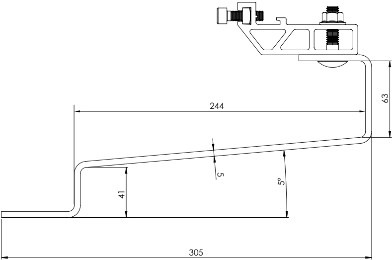
Biberschwanz Dachhaken AS 2.1
