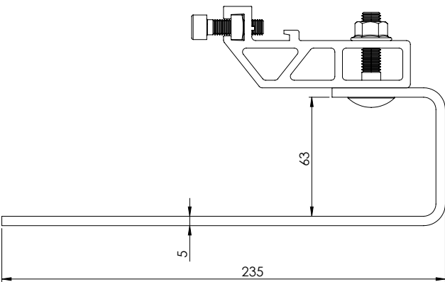
Schiefer Dachhaken AS 2.1
