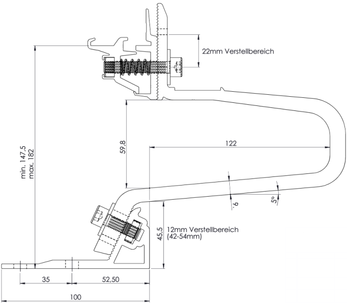
Dachhaken AL13
